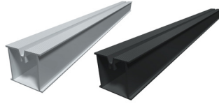
DS38 Aluminium Joist Width: 48mm Depth: 38mm Finish: Mill finish or powder coated
