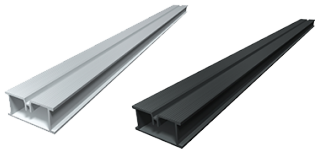
DS22 Aluminium Joist Width: 48mm Depth: 22mm Finish: Mill finish or powder coated
