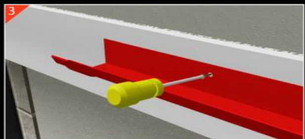
Once the position is established the first length can be fixed (level), directly through the back of the gutter using 38 x 5 stainless steel screws (Guttercrest GM1).
