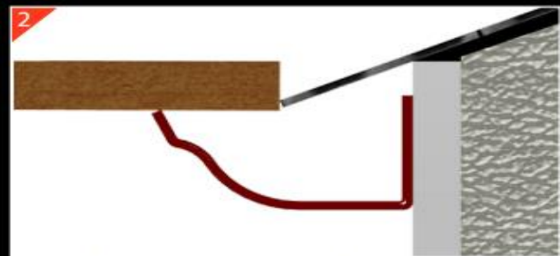
Alternatively use a spirit level against the lowest point of the roof tile to determine the position the gutter is fixed to.
