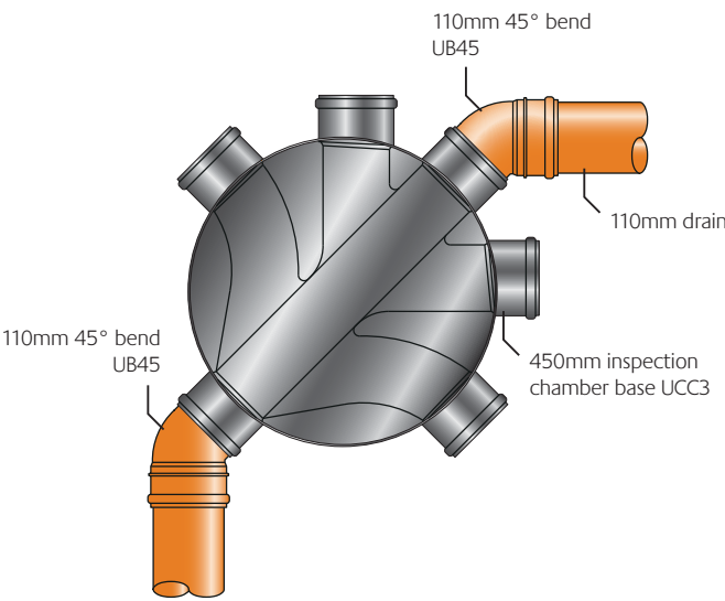
Typical 450mm inspection chamber 90° change of direction
