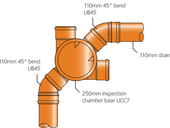
Typical 250mm inspection chamber 90° change of direction
