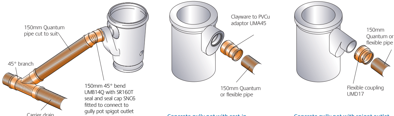
Concrete gully pot with cast-in polypropylene socket for clayware pipes
