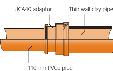
PVCu pipe socket to thin wall clayware socket
